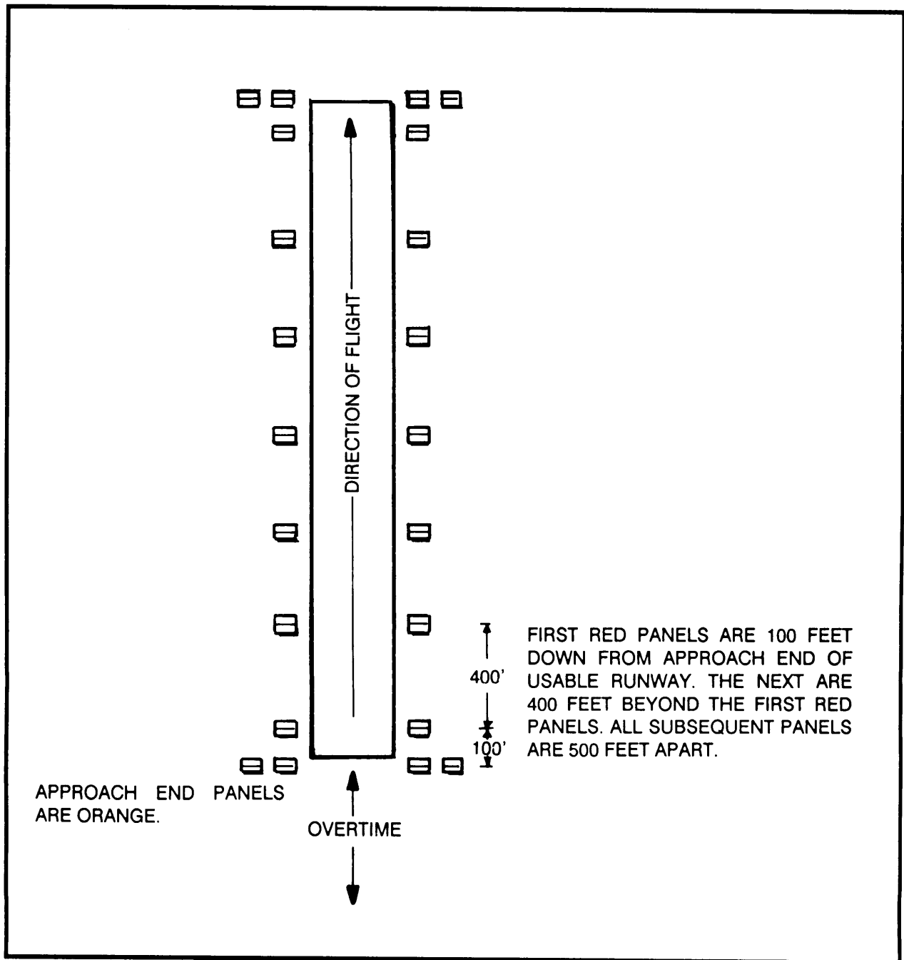
Figure A-3. Landing zone markings (day).
